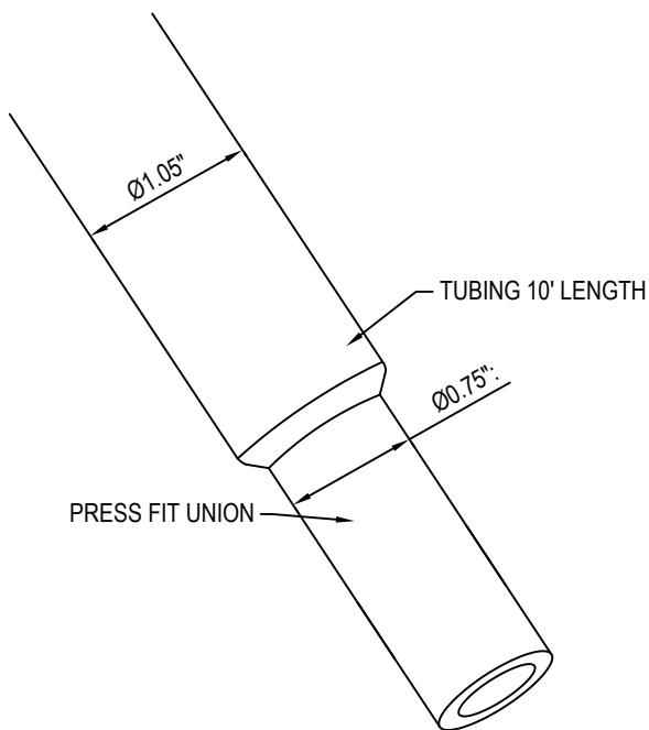
PERSPECTIVE
