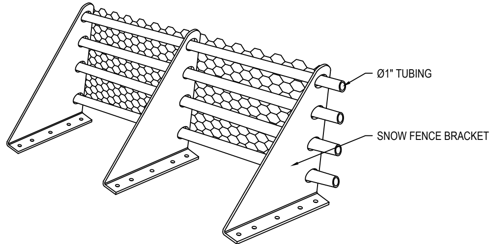
ISOMETRIC VIEW
