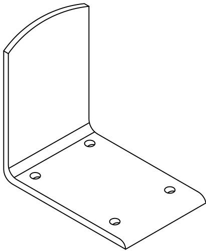
ISOMETRIC VIEW
